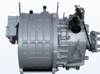
KINGLONG Brand PMSM Whose Max/Rated Power Is 80/50Kw, Max Torque Is 310 Nm; The Max. Gradient Is 25% (Full Load)
